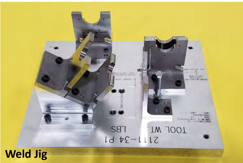
Weld Jig
