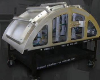
BONDING JIGS
