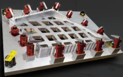
ROUTER FIXTURES
