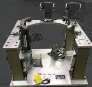
WELD JIGS
